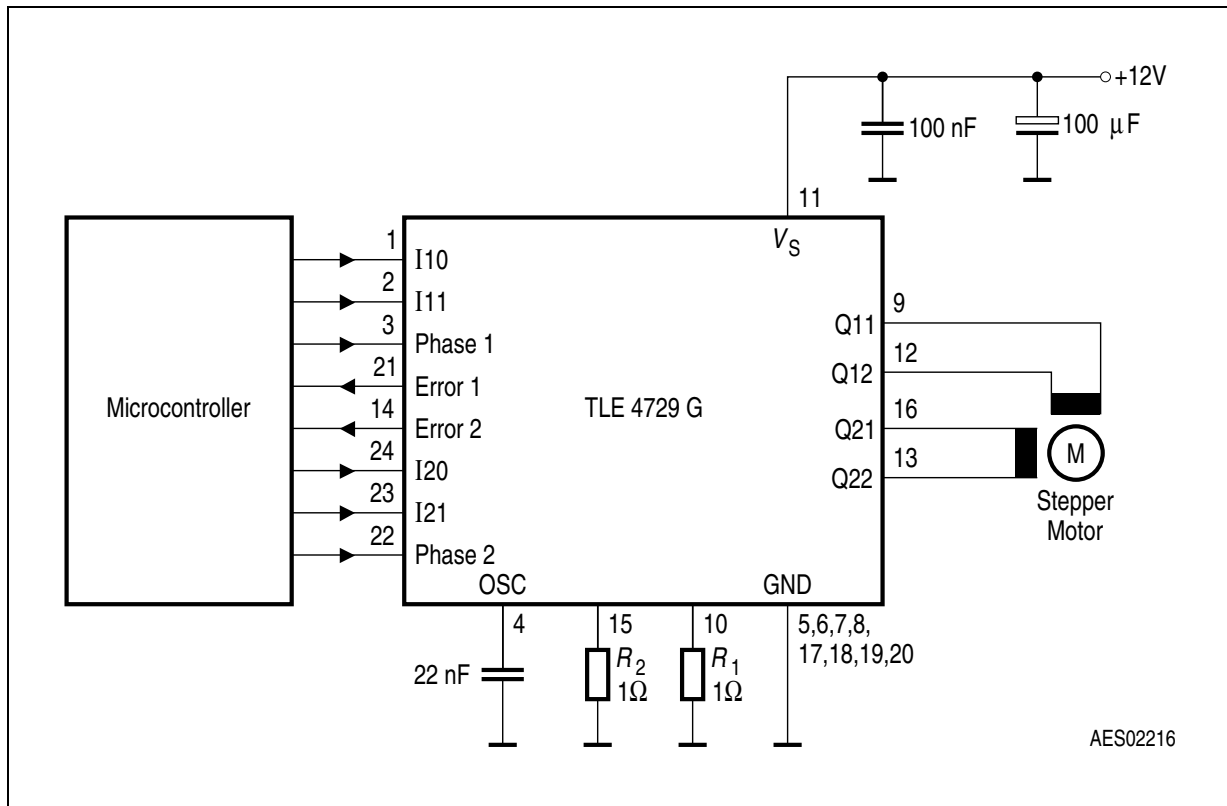
Figure 3 Application Circuit
