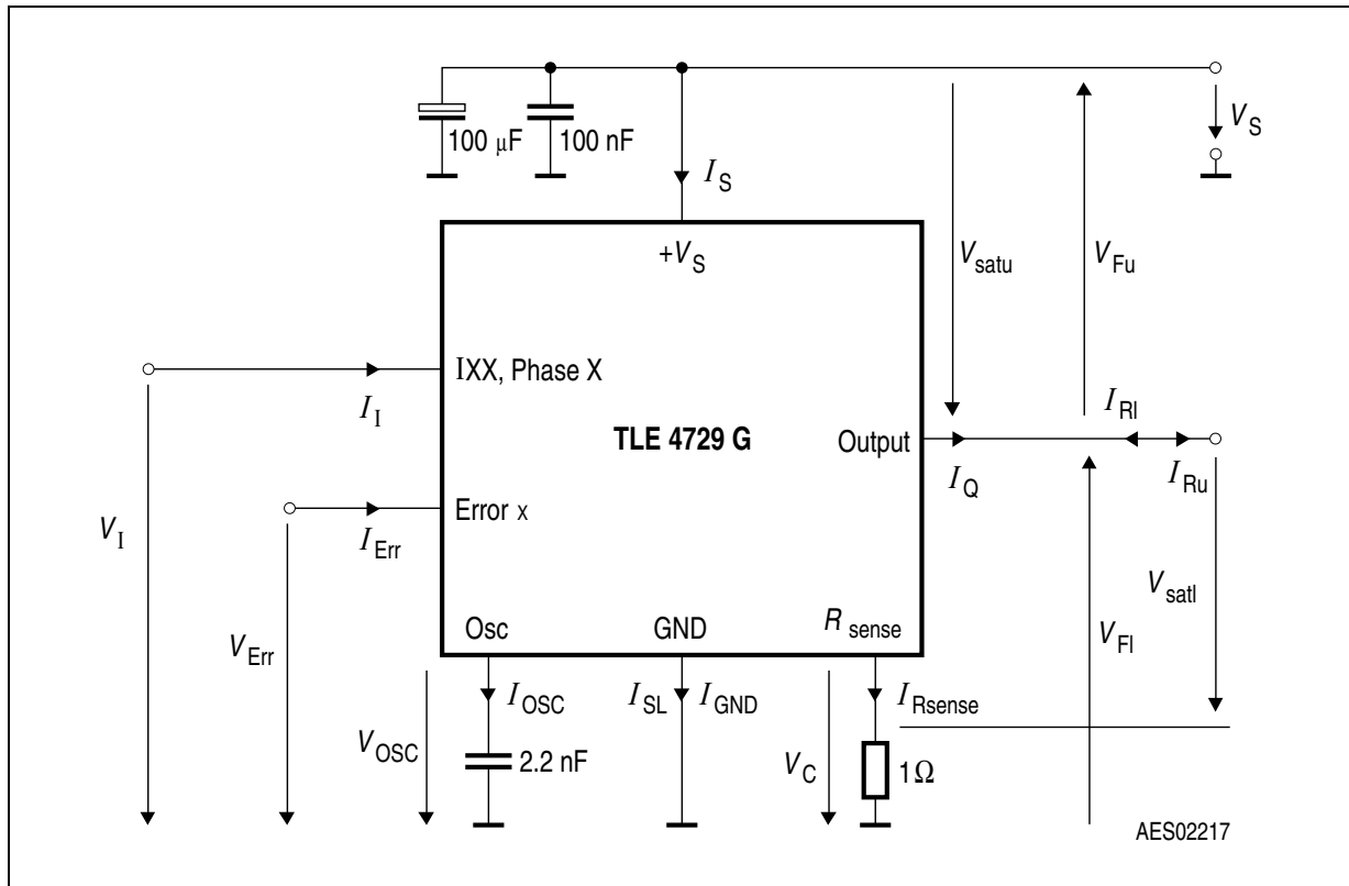
Figure 4 Test Circuit
