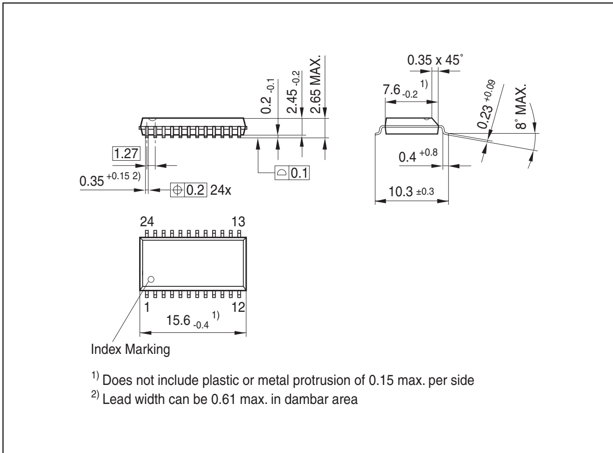
Figure 11 PG-DSO-24-16 (Plastic Green Dual Small Outline)
