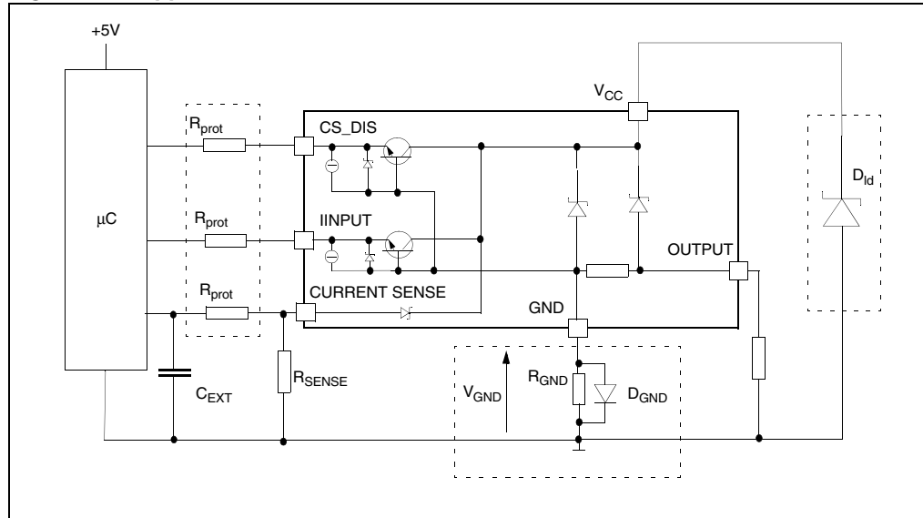
Figure 26. Application schematic
