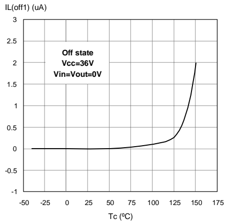
Figure 10. Off State Output Current
