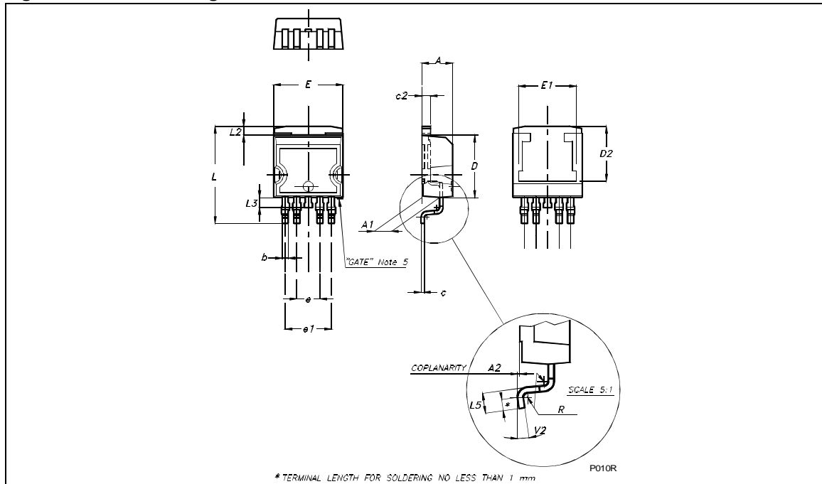
Figure 43. P 2 PAK Package Dimensions
