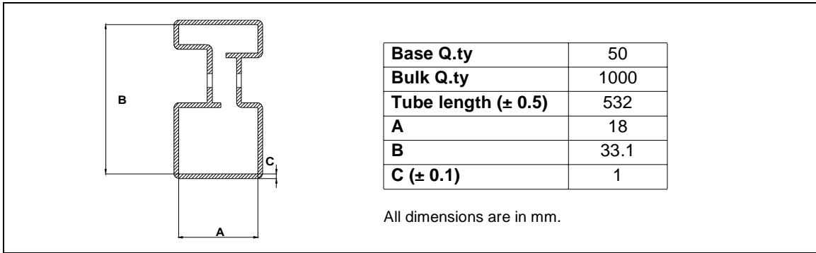
Figure 48. P 2 PAK TUBE SHIPMENT (no suffix)
