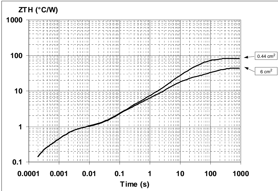
Figure 37. PPAK Thermal Impedance Junction Ambient Single Pulse
