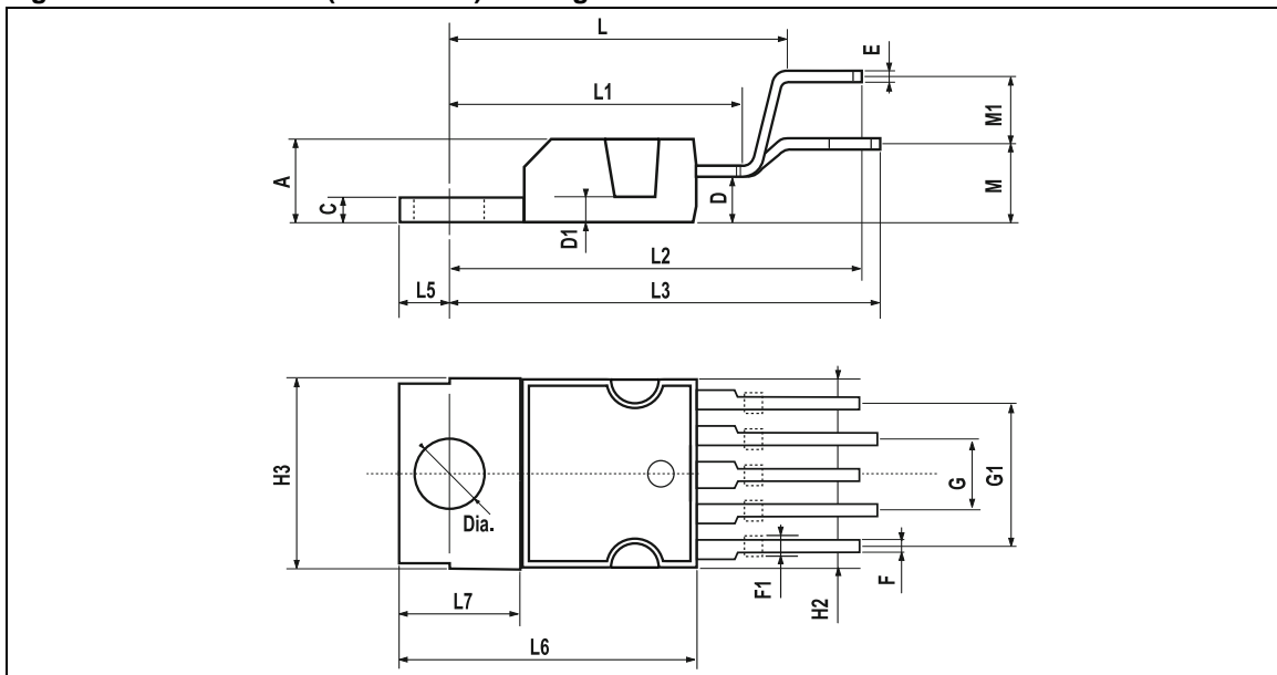
Figure 42. PENTAWATT (VERTICAL) Package Dimensions
