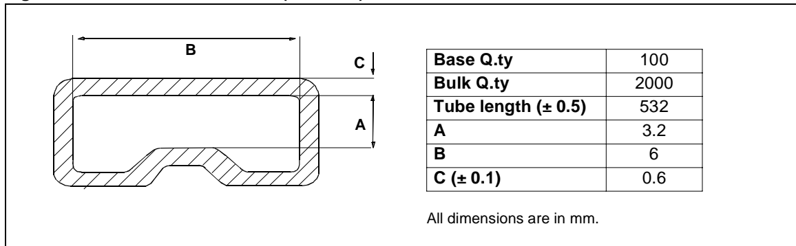
Figure 45. SO-8 TUBE SHIPMENT (no suffix)
