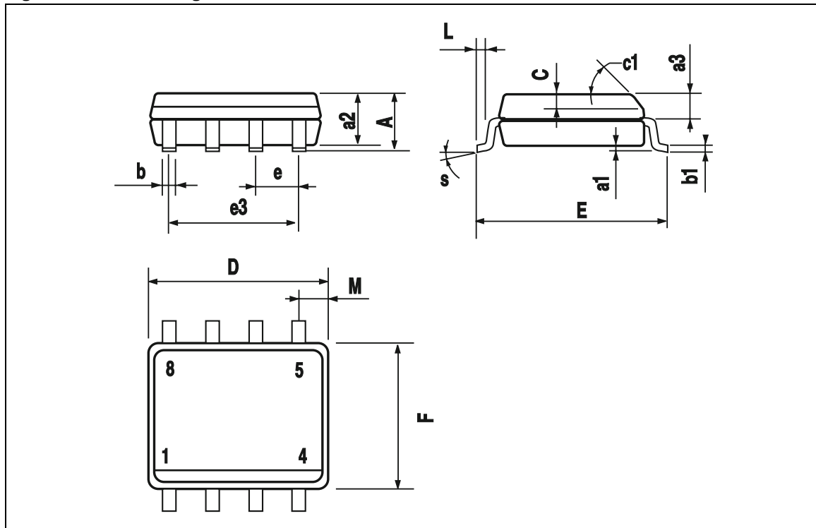
Figure 41. SO-8 Package Dimensions
