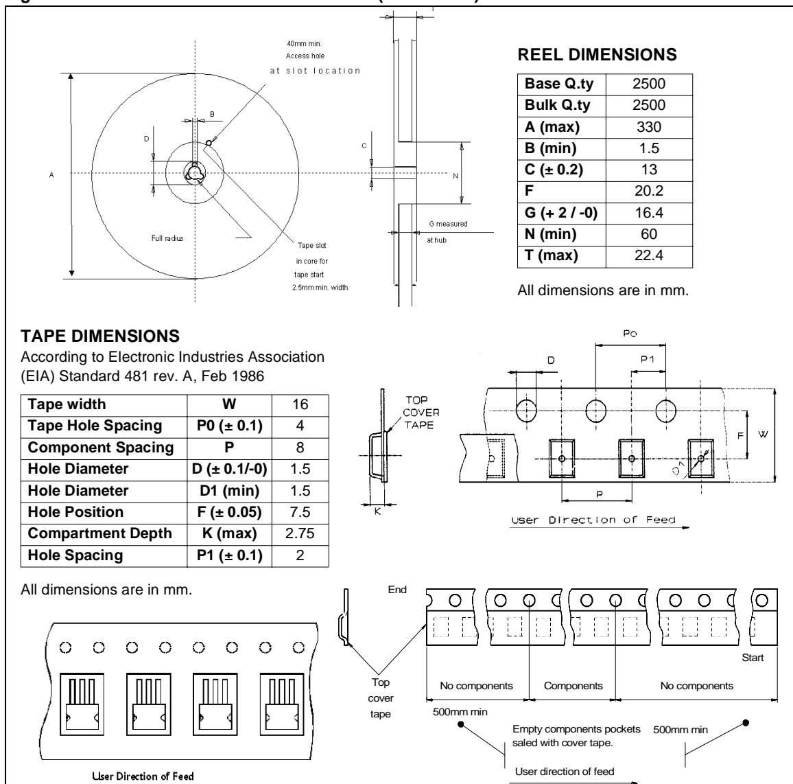
Figure 51. PPAK TAPE AND REEL SHIPMENT (suffix "TR")
