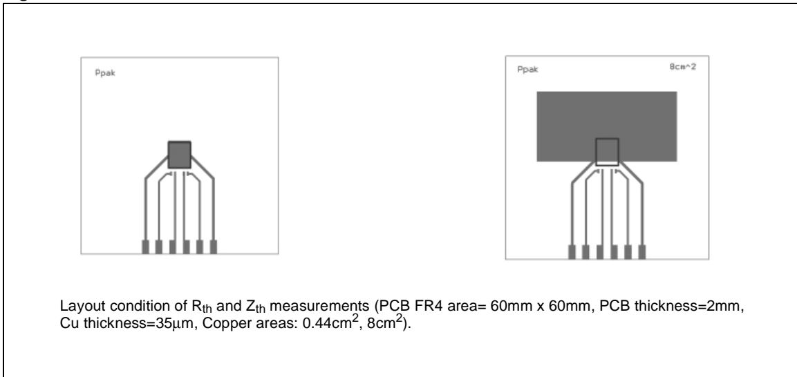
Figure 33. PPAK PC Board
