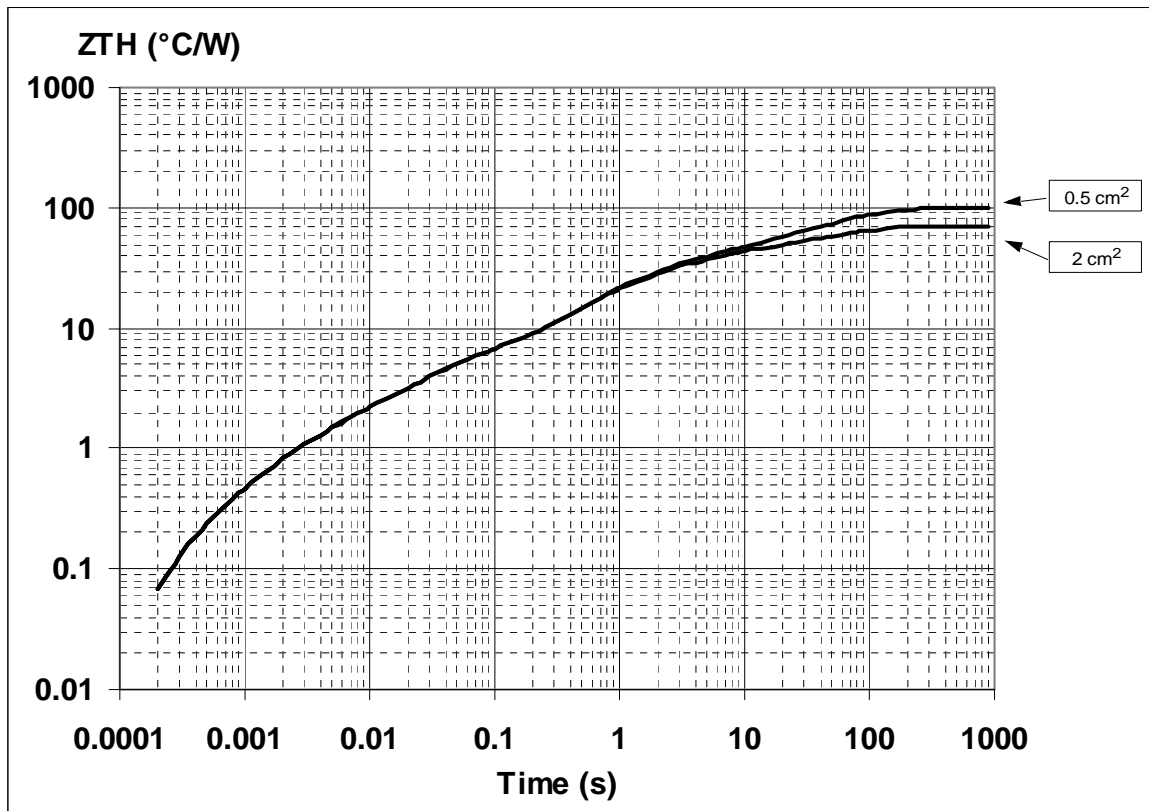
Figure 35. SO-8 Thermal Impedance Junction Ambient Single Pulse
