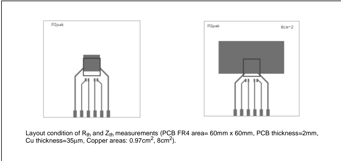
Figure 31. P 2 PAK PC Board
