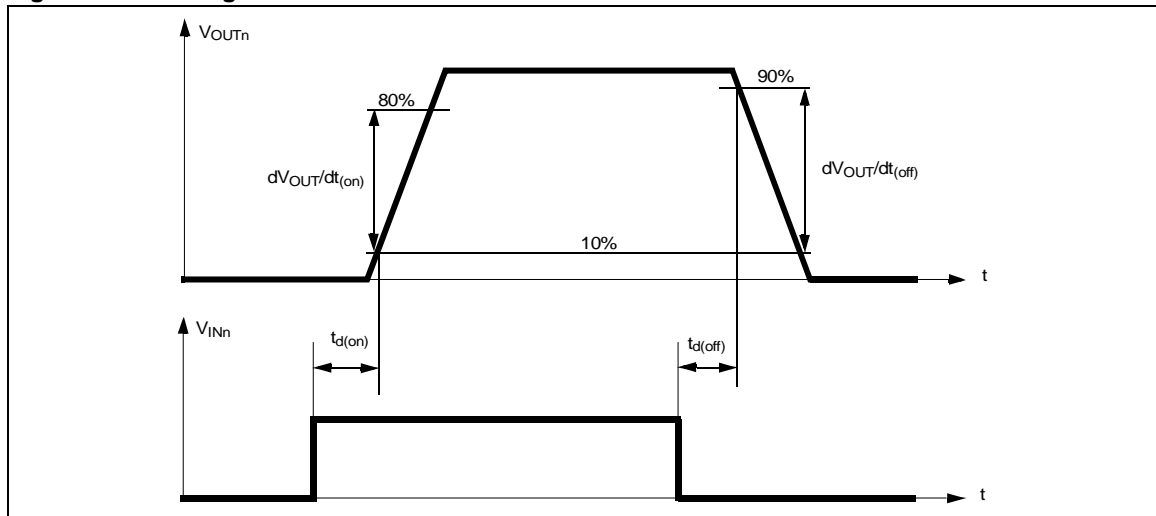
Figure 6. Switching time Waveforms
