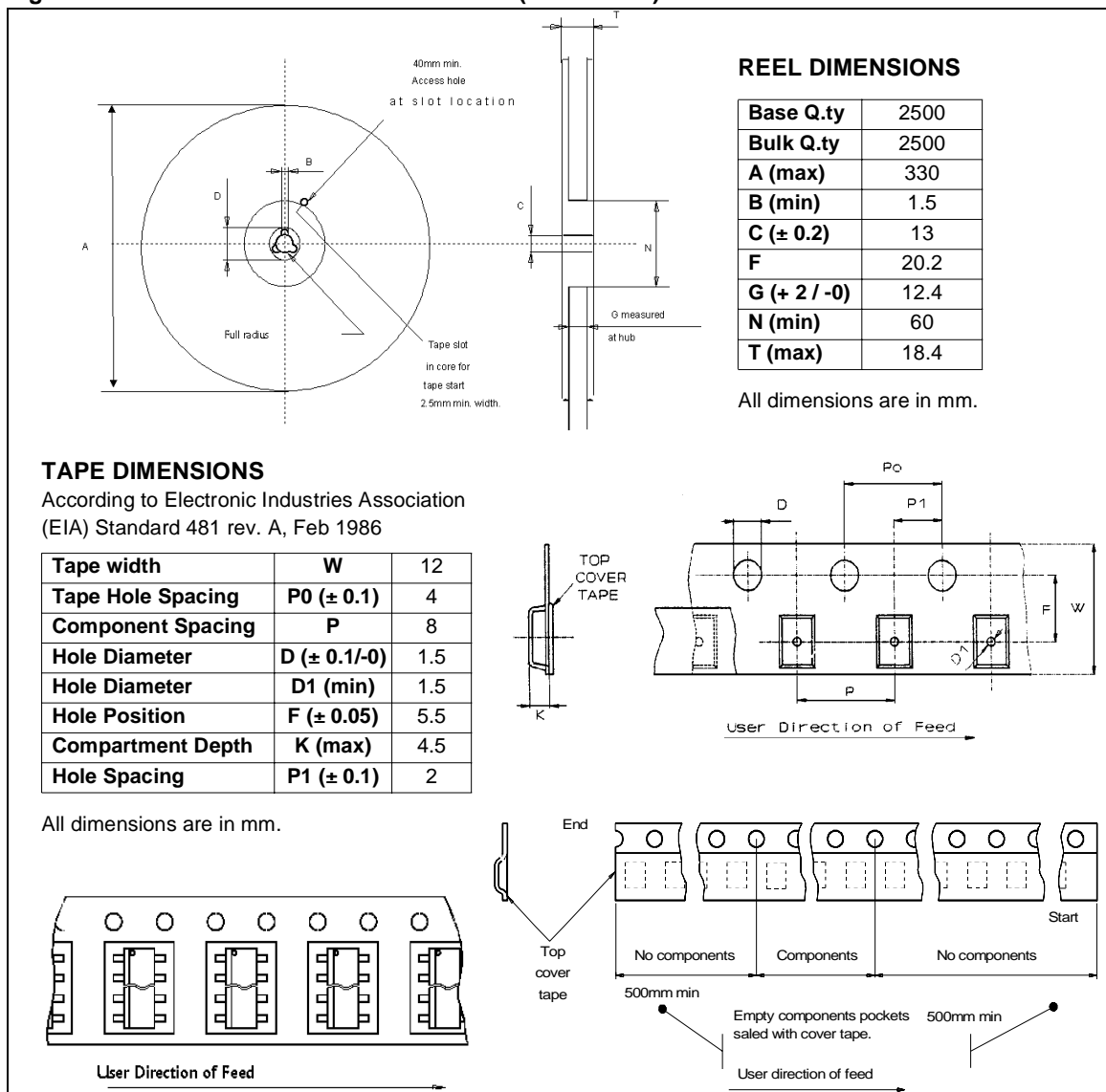
Figure 46. SO-8 TAPE AND REEL SHIPMENT (suffix "TR")
