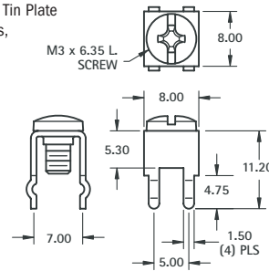
M3 VERTICAL
