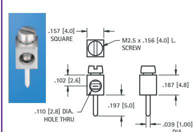
FOR .125 (3.2) BOARD
