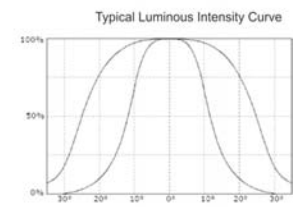
Typical Lens Efficiency: >85% - Typical Half-Divergence Angle: 12°x24°
