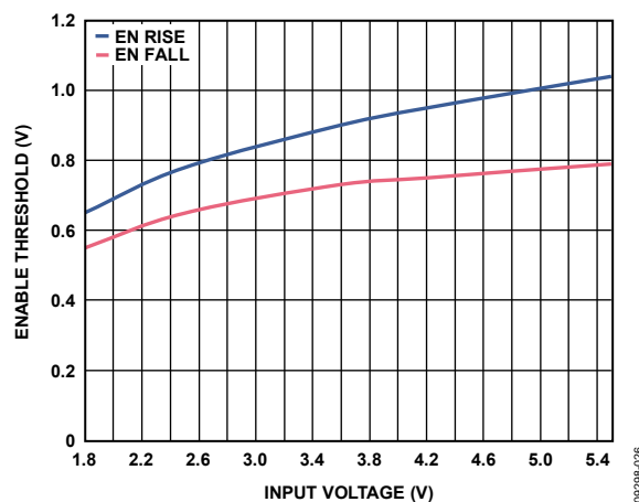
Figure 26. Typical EN Thresholds vs. Input Voltage ( V_{\text{IN}} )
