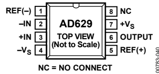
Figure 6. Pin Configuration
