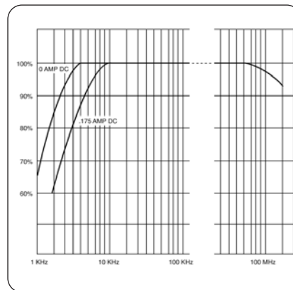
► CT2 Typical Frequency Response.
