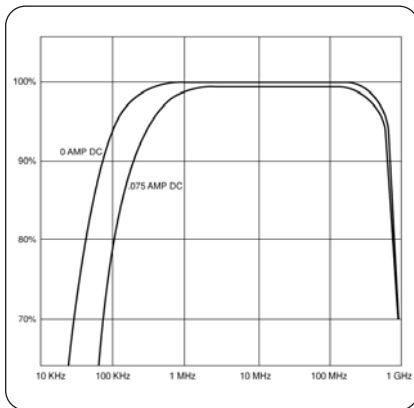
► CT1 Typical Frequency Response.
