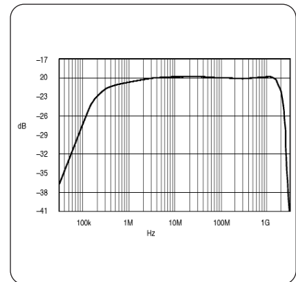
► CT6 Typical Frequency Response.
