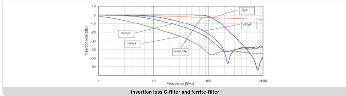
Insertion loss C-filter and ferrite-filter
