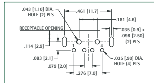
Mounting Detail
