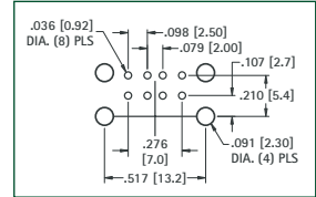
Mounting Detail
