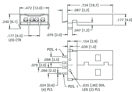
Mounting Detail
