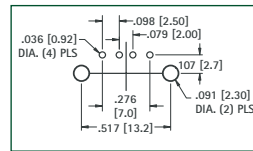
Mounting Detail
