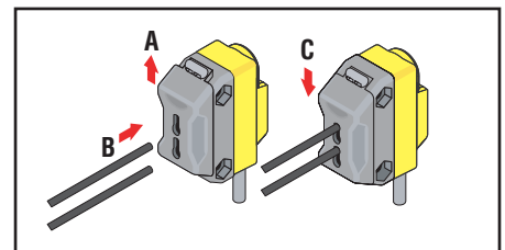
Figure 2. Installing plastic fibers
