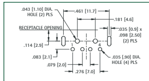
Mounting Detail
