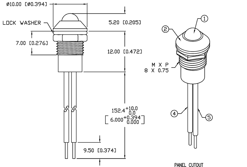
PANEL CUTOUT
