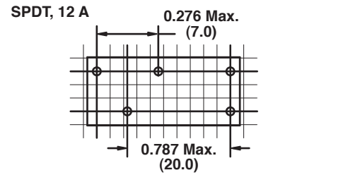
Circuit board pin spacing viewed from component side
