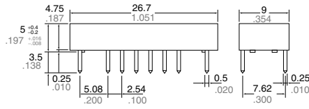
External dimensions Standard PC board terminal
