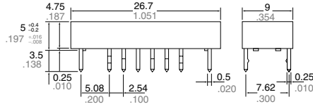
Self-clinching terminal
