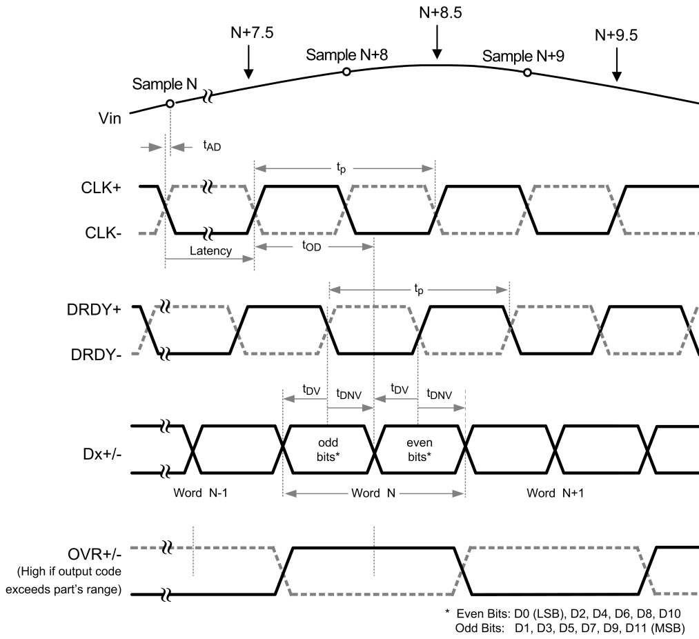
Output Timing
