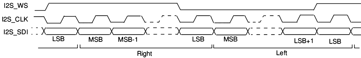
FIGURE 4. I 2 S Transmit Timing Diagram
