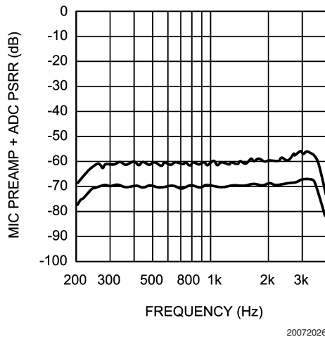
MIC PreAmp + ADC PSRR vs Frequency Top Trace = 47dB MIC Gain, Bottom Trace = 17dB MIC Gain
