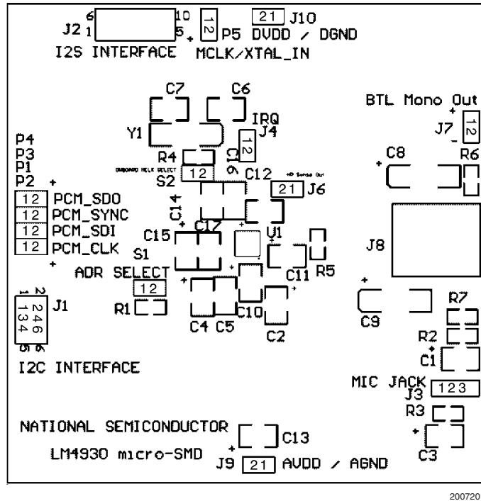
FIGURE 12. Pin Markings for LM4930ITL demo board
