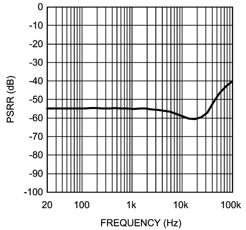
PSRR vs Frequency ( AV_{DD} = 5V, R_L = 8\Omega, \text{Handsfree Output} )
