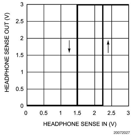
Headphone Sense In Hysteresis Loop (AV DD = 3V)
