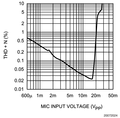
ADC THD+N vs MIC Input Voltage (MIC Gain = 47dB)
