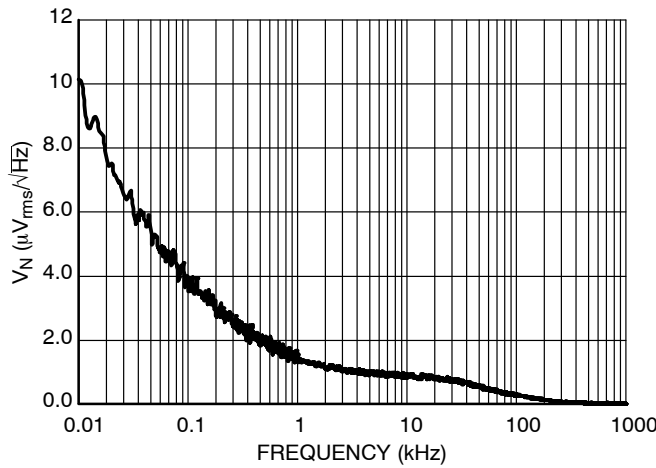
Figure 25. Output Voltage Noise, 5.0 V Version, V_{IN} = 6.0 V
