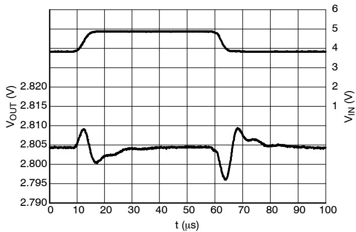
Figure 27. Line Transients, 2.8 V Version, t_R = t_F = 5 \mu s , I_{OUT} = 30 \text{ mA}
