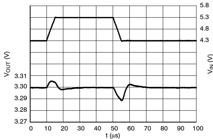
Figure 23. Line Transients, 3.3 V Version, t_R = t_F = 5 \mu\text{s} , I_{OUT} = 30 \text{ mA}
