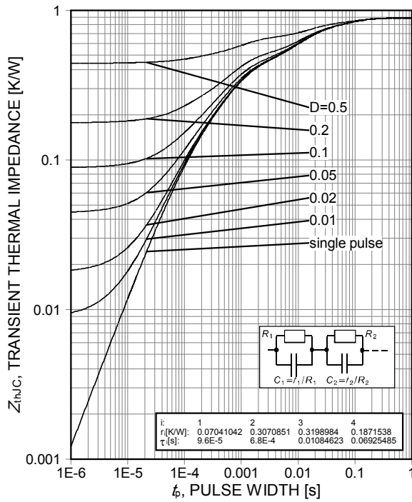
Figure 21. IGBT transient thermal impedance ( D = \phi_p / T )
