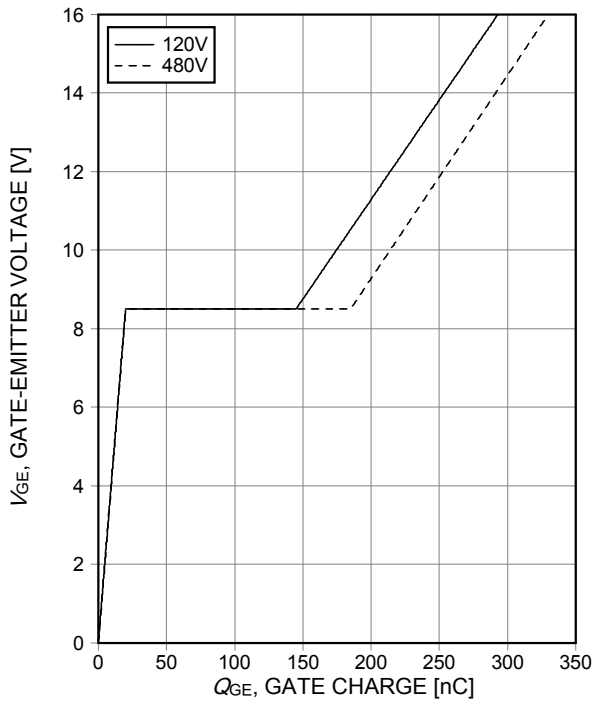
Figure 17. Typical gate charge ( I_C=50A )
