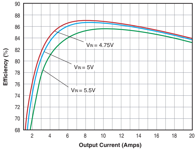
UNR-2.5/15-D5 Efficiency vs. Load @ 25°C Ambient
