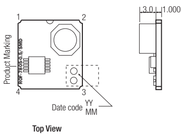
ROF-78xx-0.5SMD Surface Mount Package
