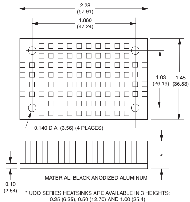
Figure 8. Optional Heatsink
