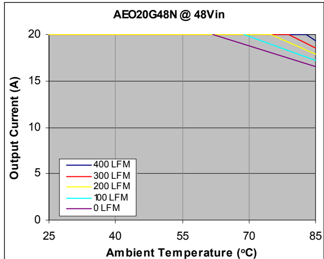
Figure 36. Output Current vs. Temperature for baseplate version at V_{IN} = 48\text{Vdc} , T_A = 25^\circ\text{C} .
