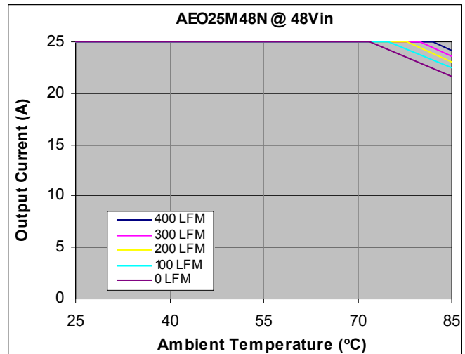
Figure 52. Output Current vs. Temperature for baseplate version at V_{\text{IN}} = 48\text{Vdc} , T_A = 25^\circ\text{C} .
