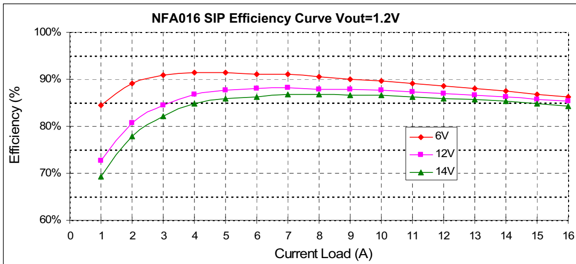
Fig 21. SIP Efficiency Curves for Vout=1.2V (25C)
