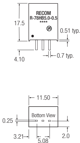
SIP3 PIN Package
