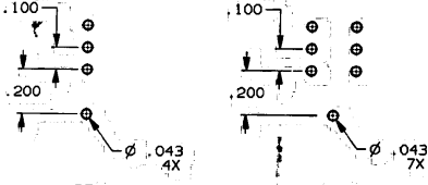
RECOMMENDED HOLE LAYOUT TOLERANCE ±.002 UNLESS OTHERWISE NOTED
