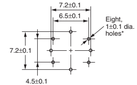
PCB Mounting (Top View)
