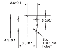
PCB Mounting (Top View)
