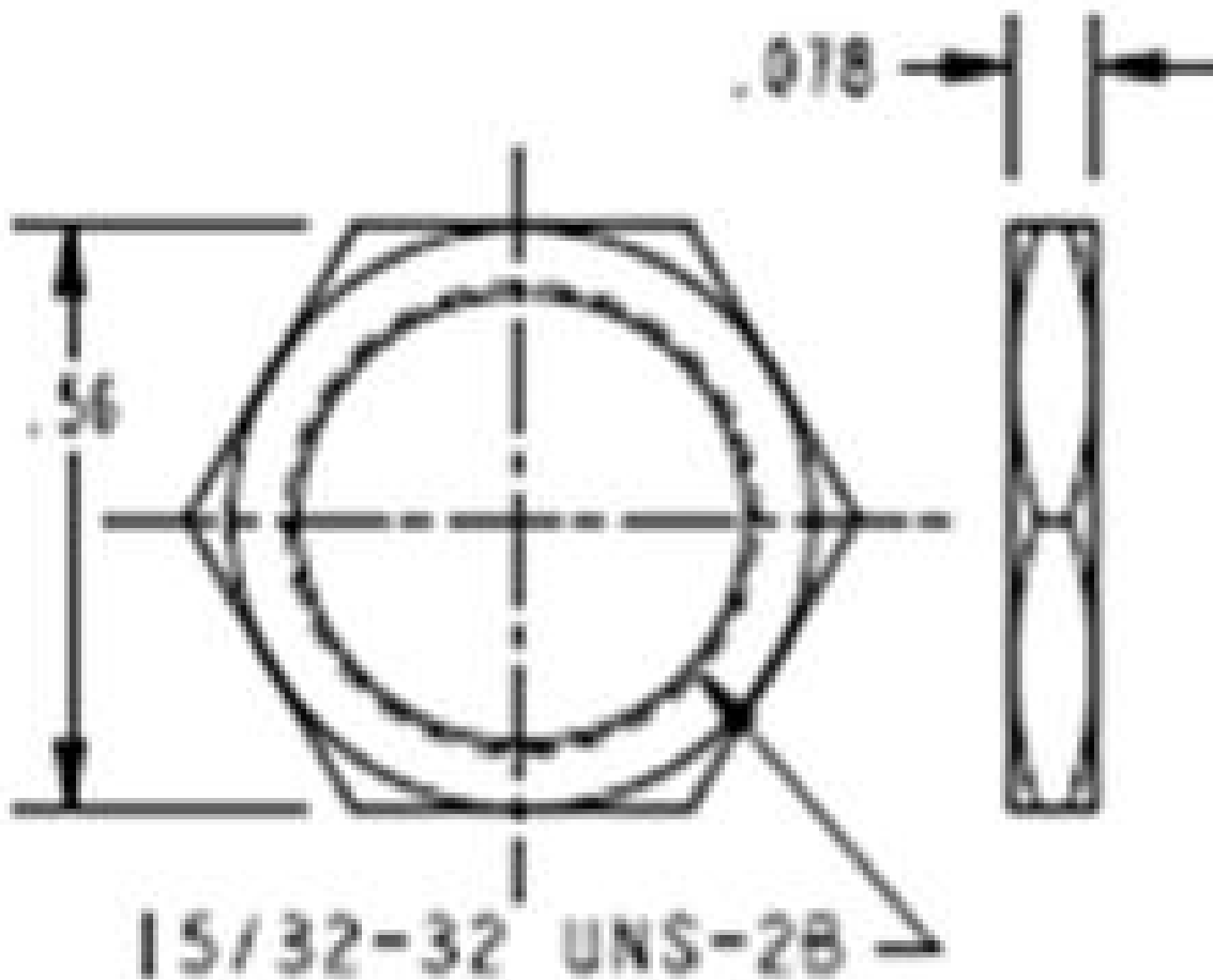
HEX NUT (PART NO. TL-11683) STEEL, ZINC COBALT PLATE
