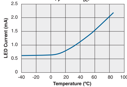
Typical I_F for Switch Dropout vs. Temperature ( I_F=170\text{mA}_{\text{DC}} )
