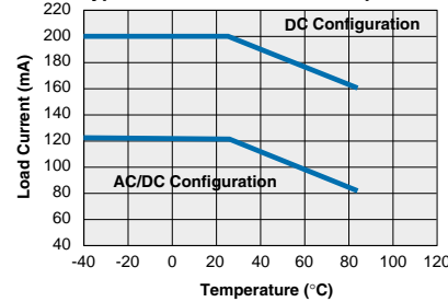
LCB110 Typical Load Current vs. Temperature
