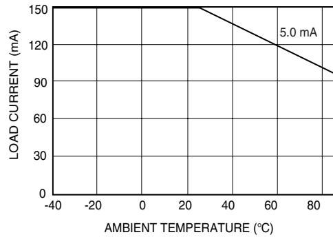
Figure 1. Recommended Operating Conditions
