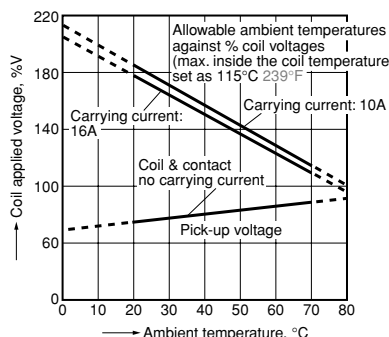
2. Ambient temperature characteristics and coil applied voltage
