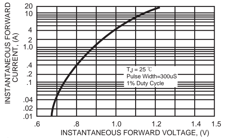
FIG. 2 - TYPICAL INSTANTANEOUS FORWARD CHARACTERISTICS
