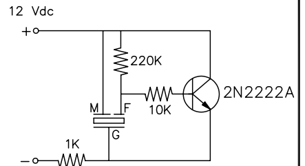
Basic Driving Circuit
