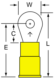
MVU10-6R Stud Size: 6 Wire Range: 12-10
