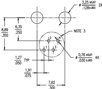
BOARD LAYOUT VIEWED FROM TOP
