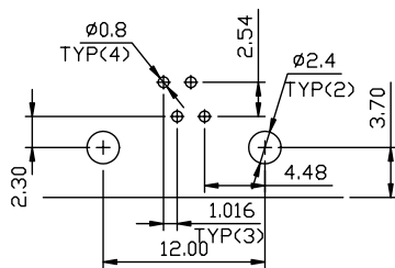
RECOMMENDED P.C.B.(.063 THK) PATTERN---4POS
