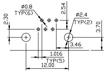
RECOMMENDED P.C.B.(.063 THK) PATTERN---6POS
