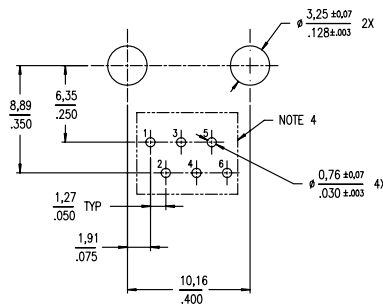
BOARD LAYOUT VIEWED FROM TOP
