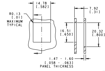
SUGGESTED FLUSH MOUNT PANEL APPLICATION CUTOY
