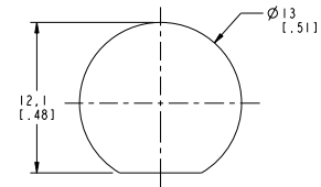
RECOMMENDED MOUNTING HOLE DIMENSIONS SCALE 3.000
