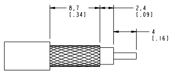
RECOMMENDED CABLE STRIPPING DIMENSIONS SCALE 3.000
