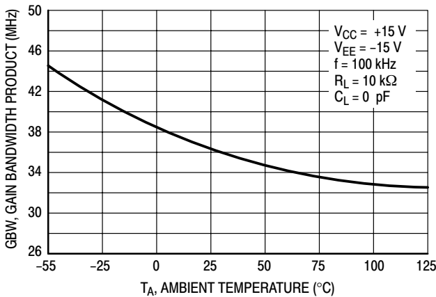
Figure 14. Gain Bandwidth Product versus Temperature
