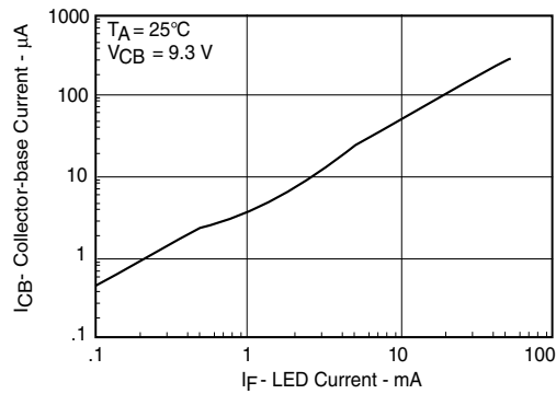
Figure 6. Collector-Base Photocurrent vs. LED Current
