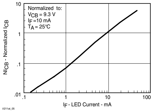
Figure 5. Normalized Collector-Base Photocurrent vs. LED Current
