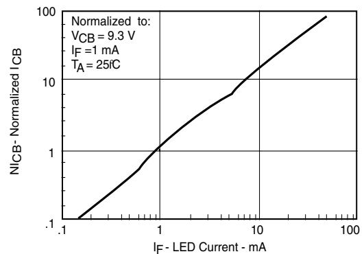
Figure 4. Normalized Collector-Base Photocurrent vs. LED Current
