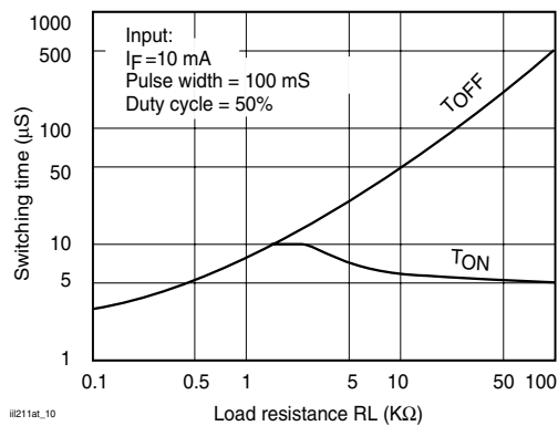
Figure 10. Typical Switching Times vs. Load Resistance
