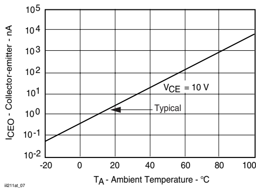
Figure 7. Collector-Emitter Leakage Current vs. Temp.
