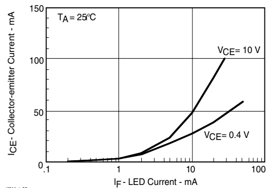
Figure 3. Collector-Emitter Current vs. LED Current
