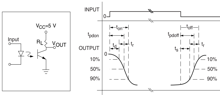
Figure 11. Switching Test Circuit
