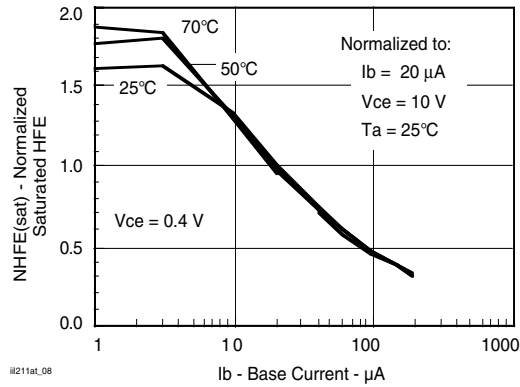
Figure 8. Normalized Saturated HFE vs. Base Current and Temperature
