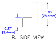
R. SIDE VIEW
