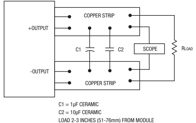
Figure 5: Measuring Output Ripple and Noise (PAR)
