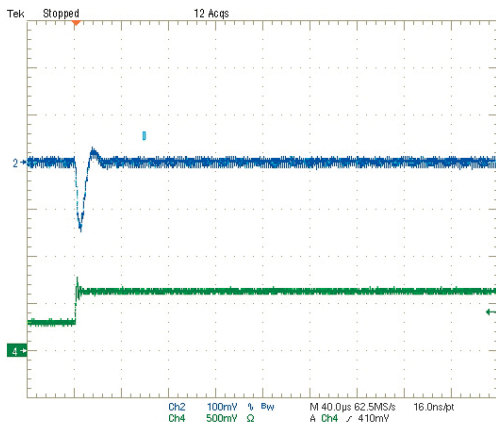
Step Load Transient Response (Vin=5V, Vout=1.2V, Clod=0, Iout=1.5A to 3A) Trace 2=Vout, 100 mV/div. Trace 4=Iout, 2.5A/div.
