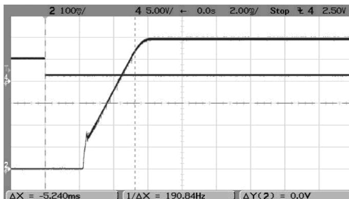
Step Load Transient Response (Vin=5V, Vout=0.6V, Load=0, Iout=3A to 1.5A) Trace 2=Vout, 100 mV/div. Trace 4=Iout, 2.5A/div.
