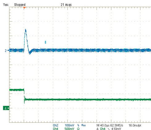
Step Load Transient Response (Vin=5V, Vout=1.5V, Clod=0, Iout=3A to 1.5A) Trace 2=Vout, 100 mV/div. Trace 4=Iout, 2.5A/div.
