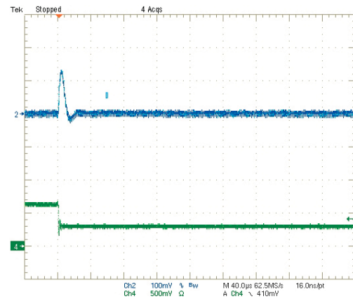
Step Load Transient Response (Vin=5V, Vout=1.2V, Clod=0, Iout=3A to 1.5A) Trace 2=Vout, 100 mV/div. Trace 4=Iout, 2.5A/div.
