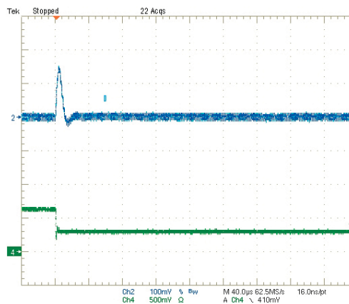
Step Load Transient Response (Vin=5V, Vout=1.8V, Clod=0, Iout=3A to 1.5A) Trace 2=Vout, 100 mV/div. Trace 4=Iout, 2.5A/div.
