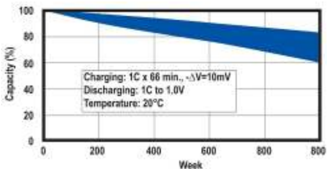
Cycle Life Using Trickle Charging
