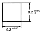
Panel Cutout of B32-12□0
