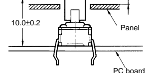
Panel Cutout of B32-13□0
